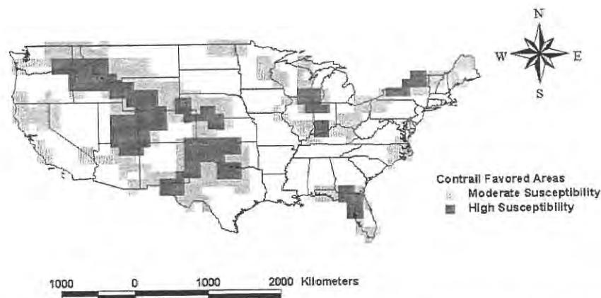
FIG. 7. Grid cell-averaged ( 1^\circ \times 1^\circ resolution) map of CFAs determined for the grounding period (1800 UTC 11 Sep 2001–1800 UTC 14 Sep 2001) using the contrail-outbreak retrodiction method applied to the six-hourly NCEP–NCAR reanalyses of the upper troposphere (refer to text). The lighter (darker) shading refers to moderate (highest) susceptibility of contrail outbreaks. Those regions that were not susceptible to outbreaks are not shaded.
